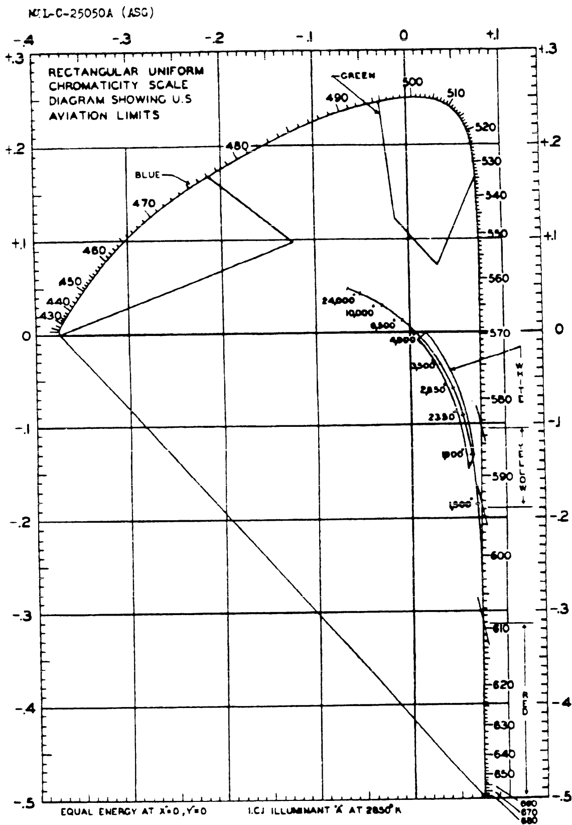
FIGURE 3. R.U.C.S. Mixture diagram showing aviation color limits
